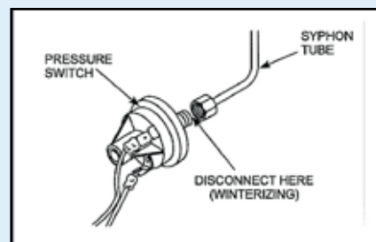
PRESSURE SWITCH
