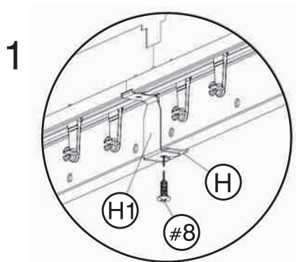
1: Remove the Joint Cover (H1)
