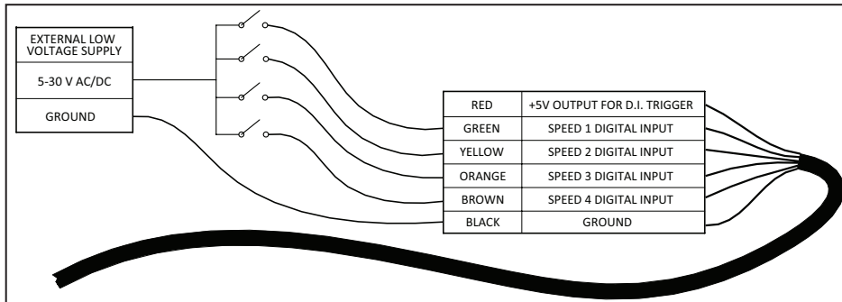
Figure 5: Low Voltage Power Supply Wiring Diagram
