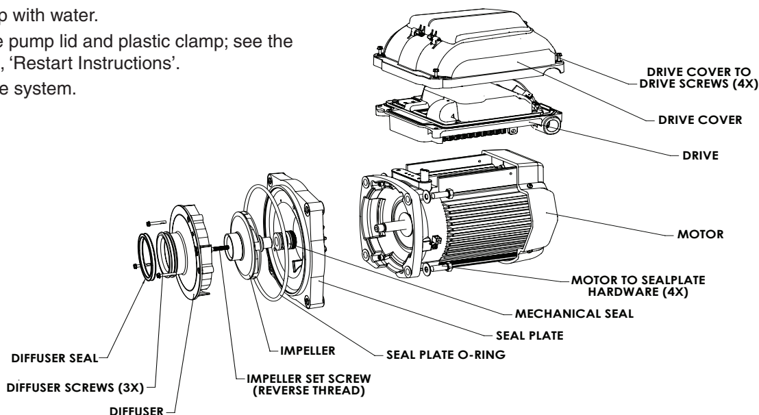
Motor Assembly
